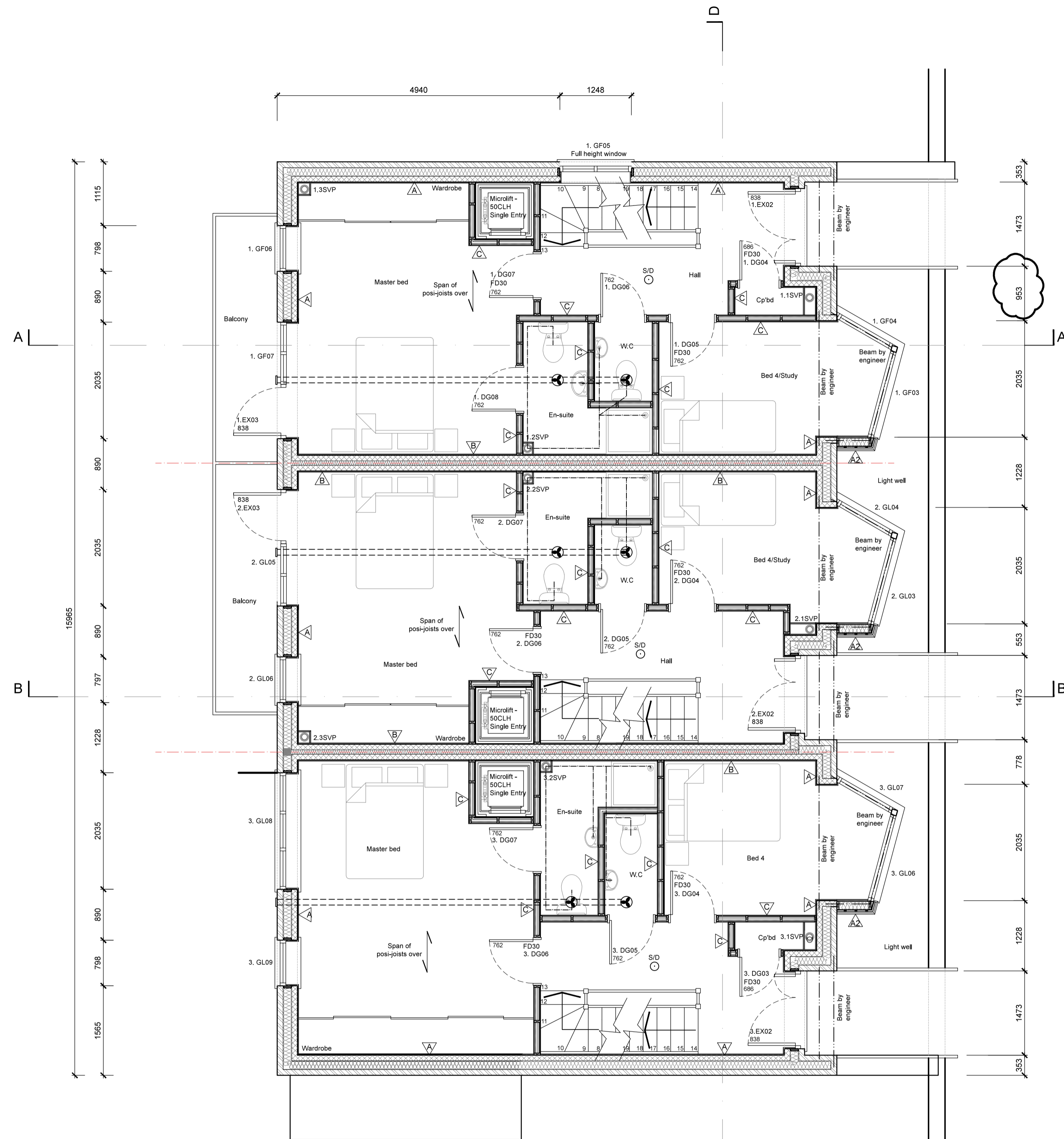
Entrance Floor Plan
