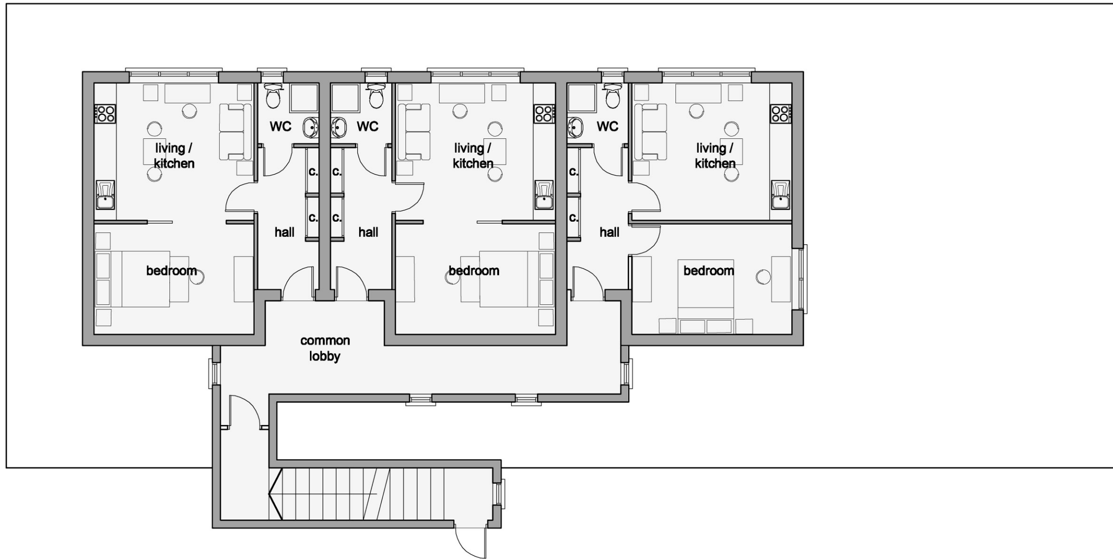
PROPOSED FIRST FLOOR PLAN RETAIL UNIT 1:100
